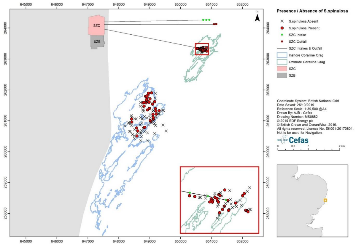
Figure 2.1: Extent of the inshore and offshore Coralline Crag and the location of ground-truthing sampling stations. Sabellaria spinulosa aggregations were identified from the acoustic image footage at both sites (red points).
